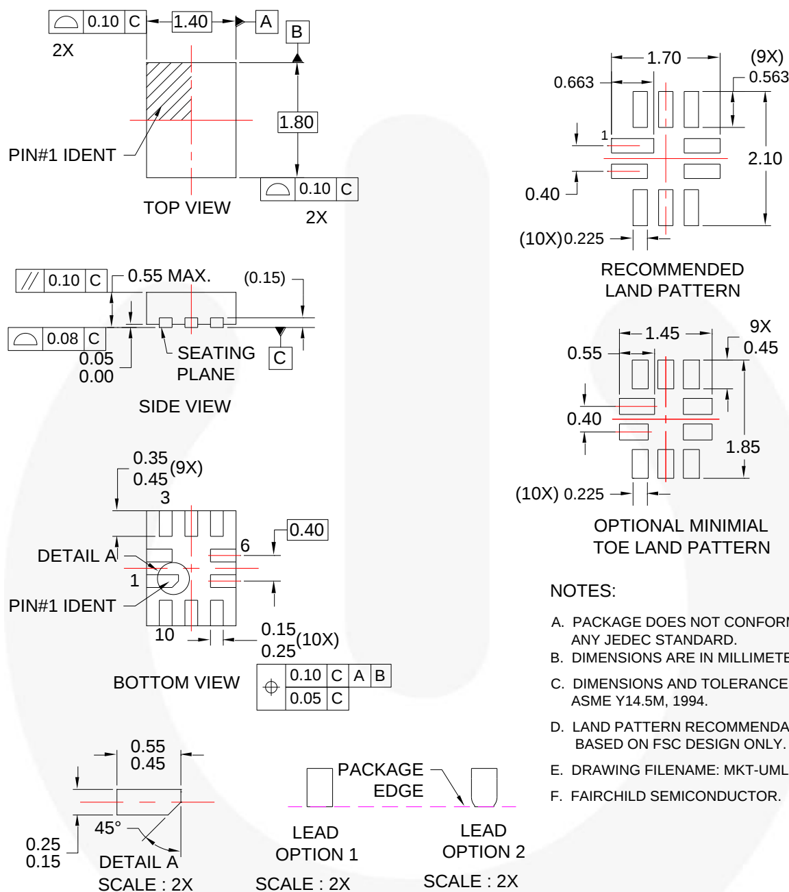
Figure 17. 10-Lead Ultrathin Molded Leadless Package (UMLP)
