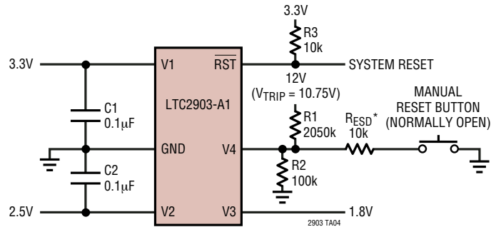
Quad Supply Monitor with Manual Reset Button
