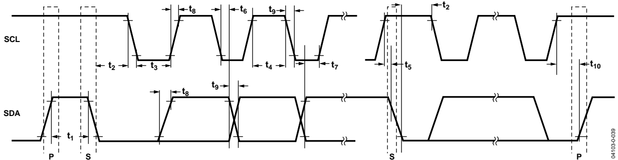
Figure 49. I 2 C Interface Detailed Timing Diagram
