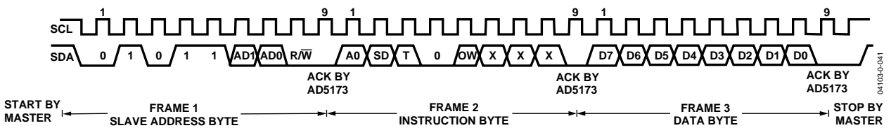
Figure 51. Writing to the RDAC Register—AD5173
