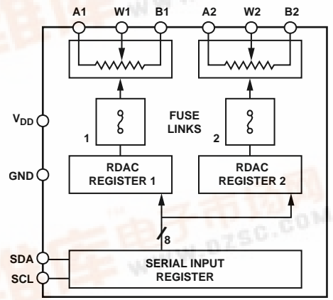
Figure 1. AD5172
