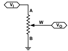
Figure 38. Potentiometer Mode Configuration
