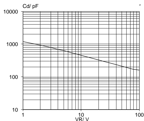
Fig.5. Typical junction capacitance per diode; C_d = f(V_R) ; f = 1 \text{ MHz} ; T_j = 25^\circ\text{C} to 125^\circ\text{C} .
